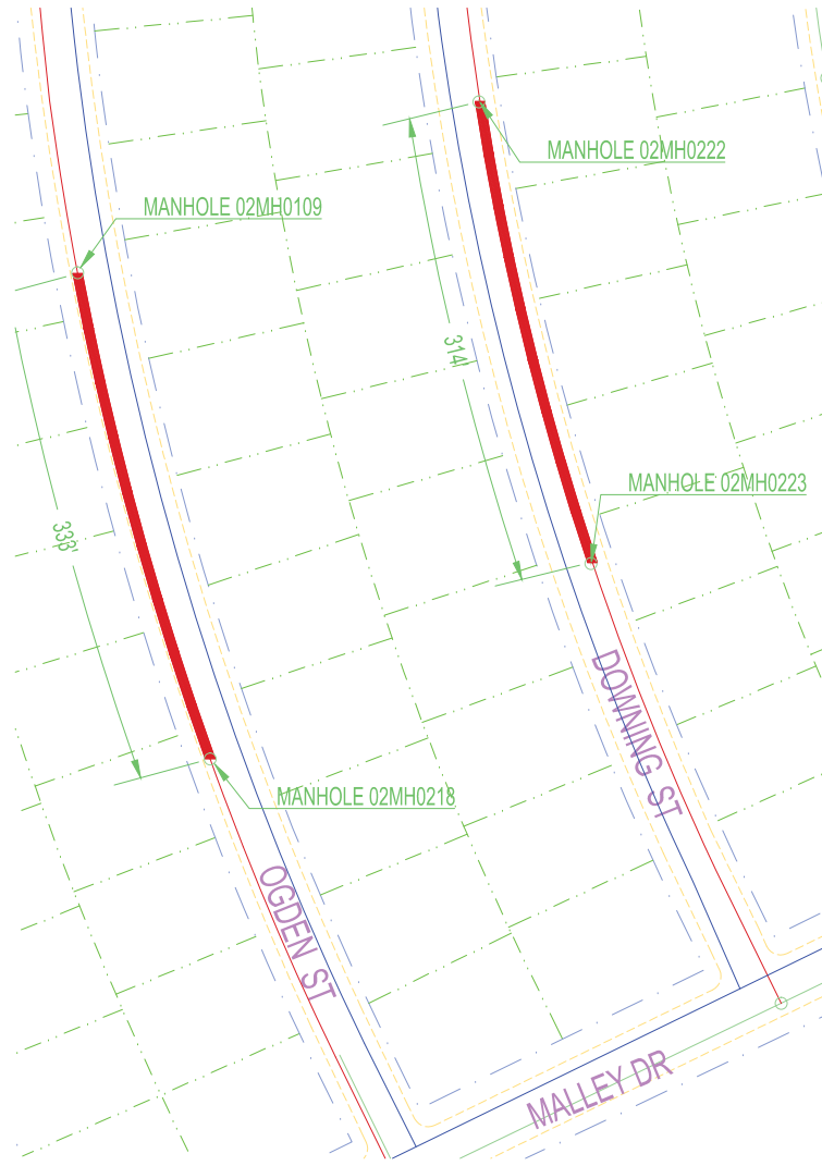
ODGEN ST AND DOWNING ST 8" SANITARY SEWER N.T.S.
