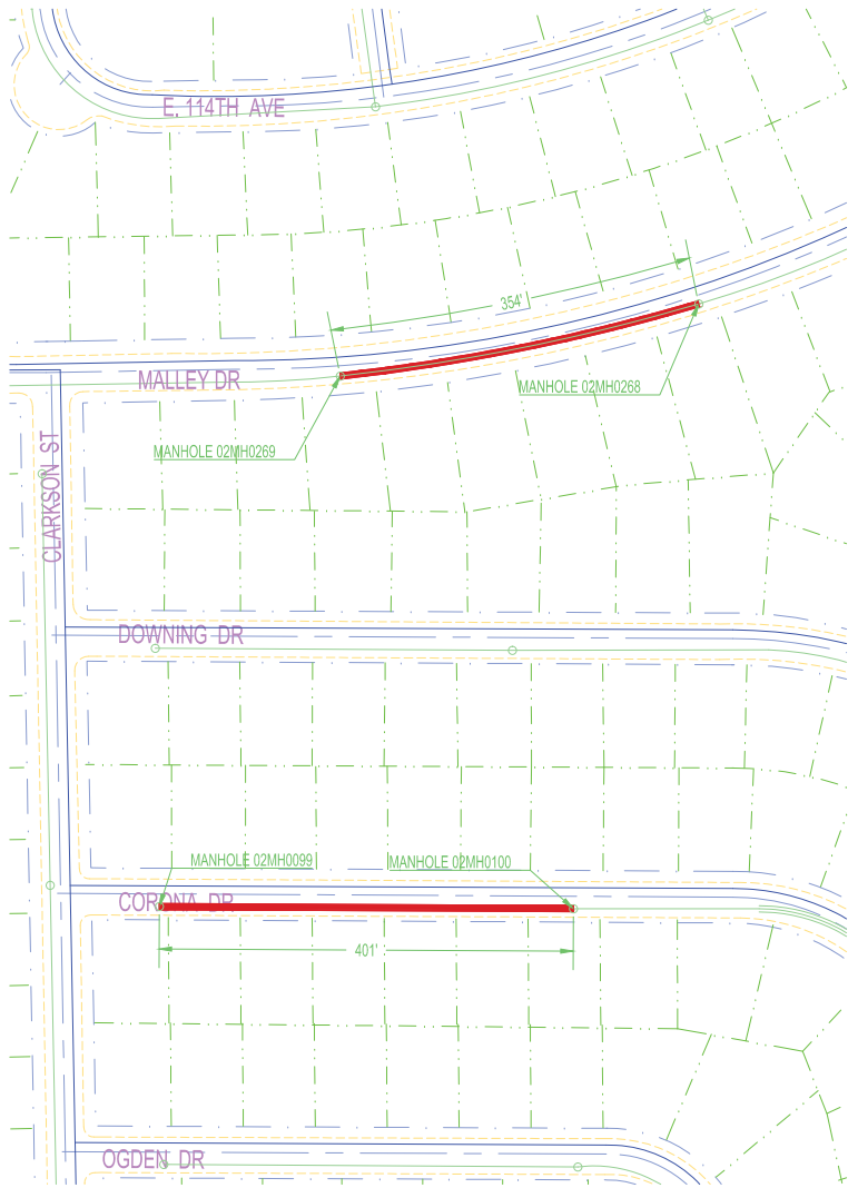
MALLEY DR AND CORONA DR 8" SANITARY SEWER N.T.S.
