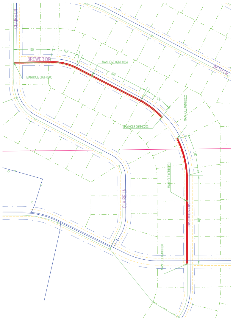
BREWER DR 8" SANITARY SEWER N.T.S.
