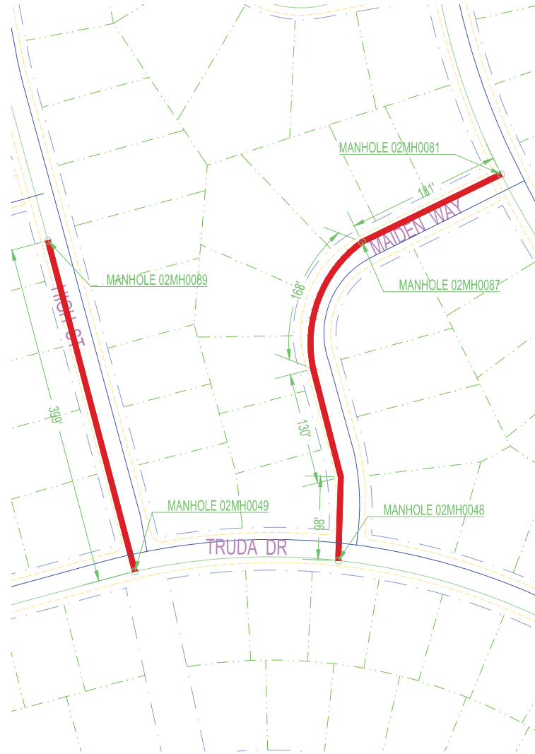
HIGH ST AND MAIDEN WAY 8" SANITARY SEWER N.T.S.
