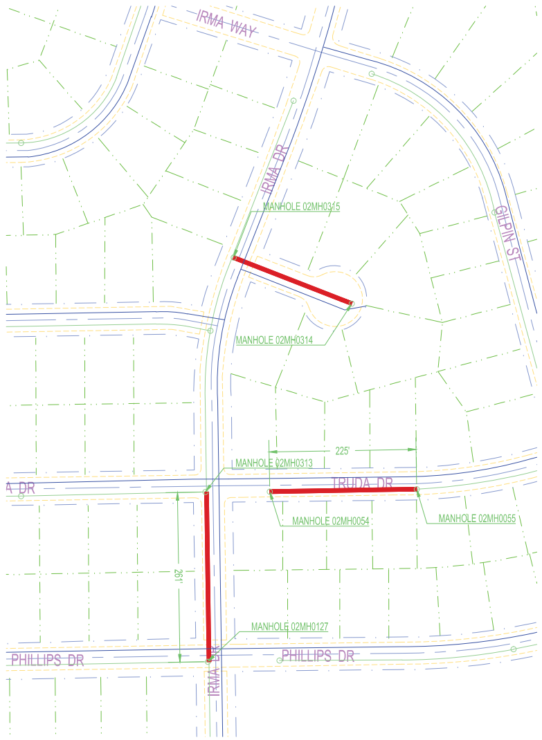
IRMA DR AND TRUDA DR 8" SANITARY SEWER N.T.S.
