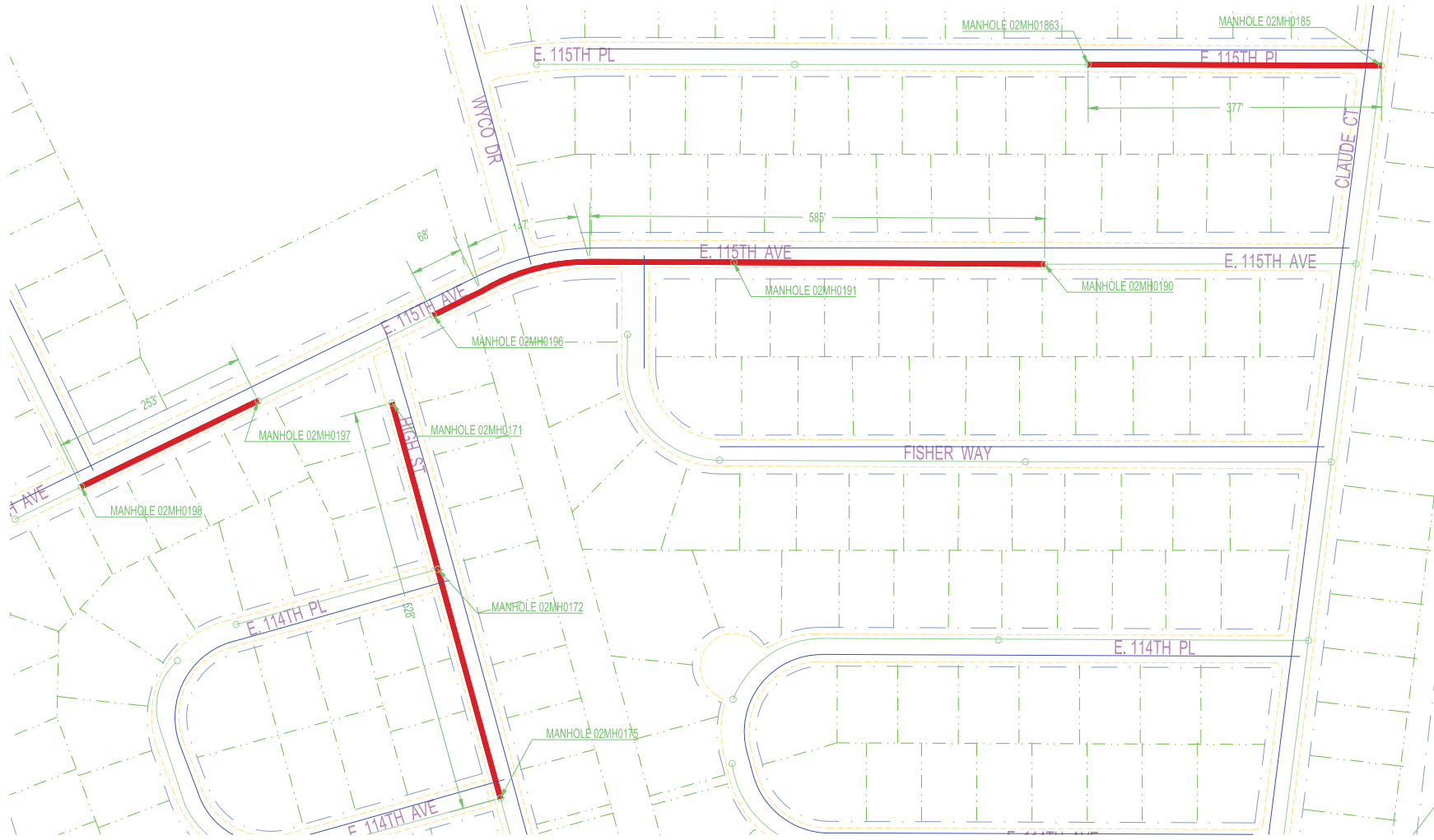
E 115TH AVE, E 115TH PL AND HIGH ST 8" SANITARY SEWER N.T.S.
