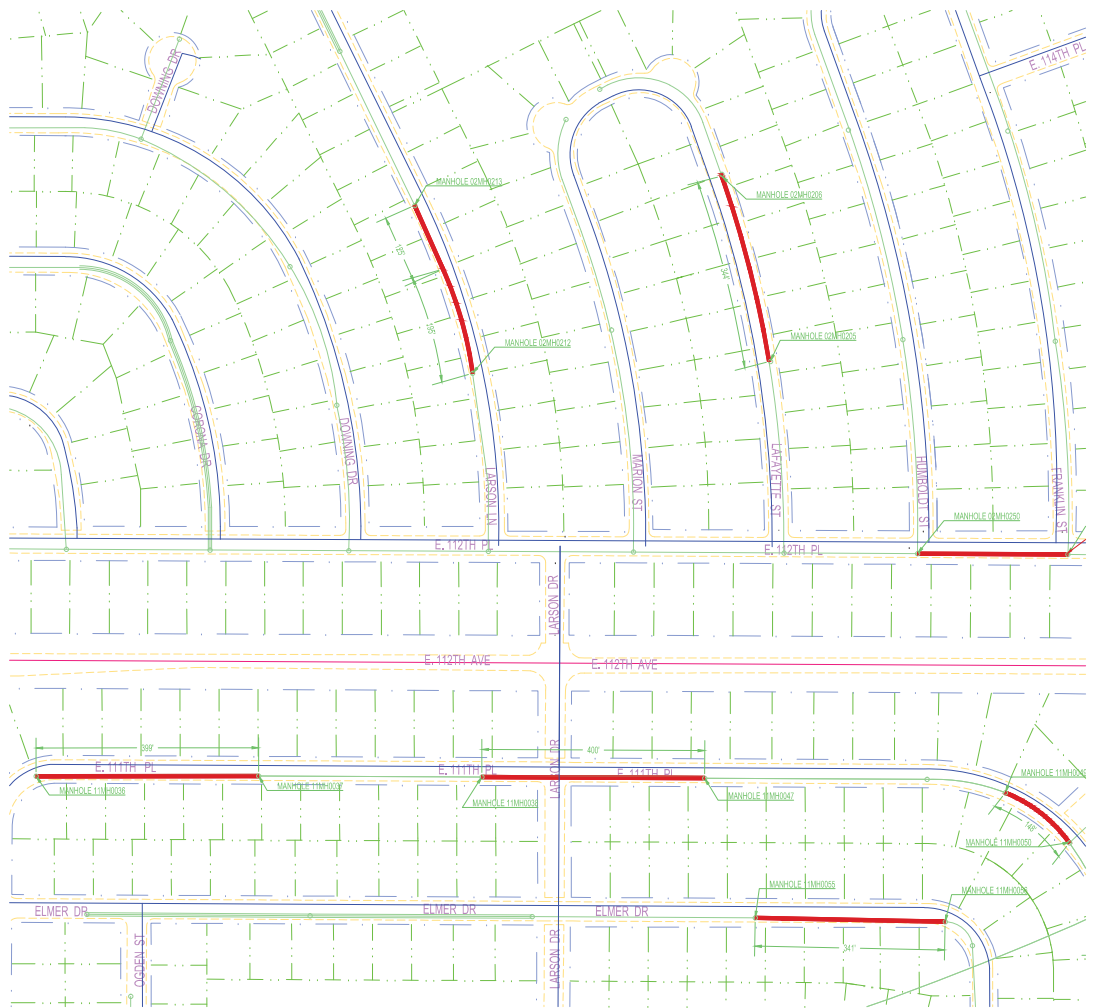
E 111TH PL, ELMER DR, LARSON LN AND LAFAYETTE ST 8" SANITARY SEWER N.T.S.
