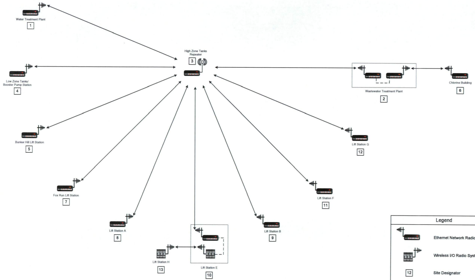
RADIO SYSTEM ARCHITECTURE No Scale
