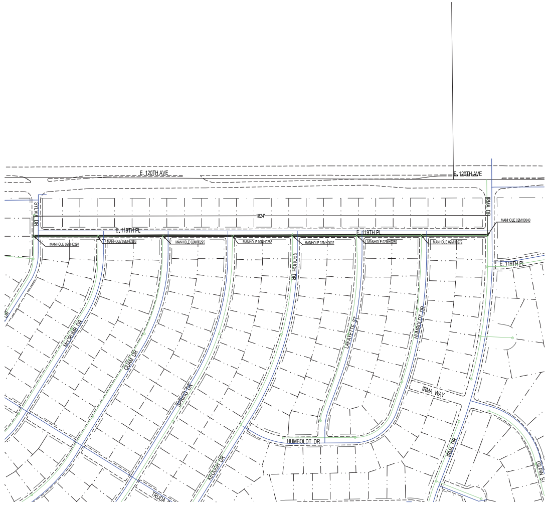
E 119TH PL 8" SANITARY SEWER N.T.S.
