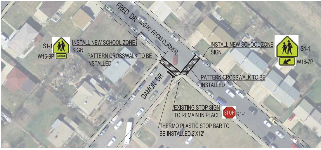
DAMON DR AND FRED INTERSECTION
