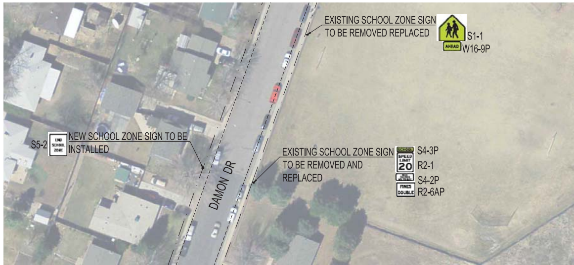
DAMON DR DETAIL 2
