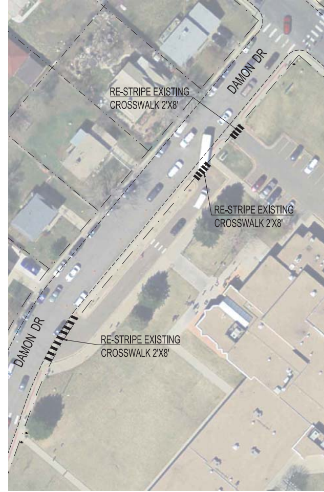
BID ALT - CROSSWALK STRIPING DAMON DR
