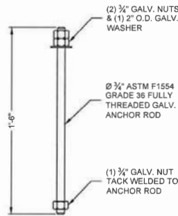
ANCHOR ROD DETAIL (8) REQUIRED SUPPLIED BY OTHERS
