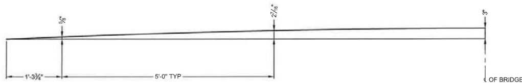
SHOP CAMBER DIAGRAM
