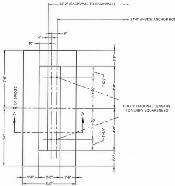
ABUTMENT PLAN
